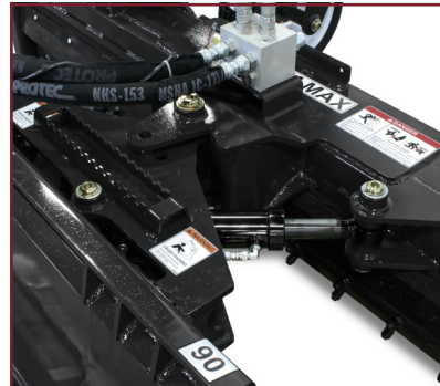
OPTION: HYDRAULIC ANGLE Angle the rake 25° left or right from inside the cab. Hydraulic Angle requires electric control option.
